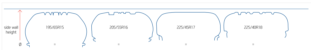
Profile comparisons of 4 tyres that have approximately the same rolling radius
